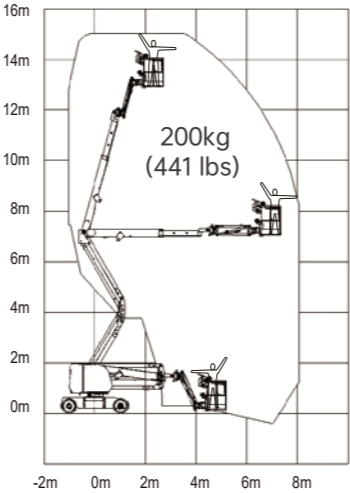
A13JE Working Range
