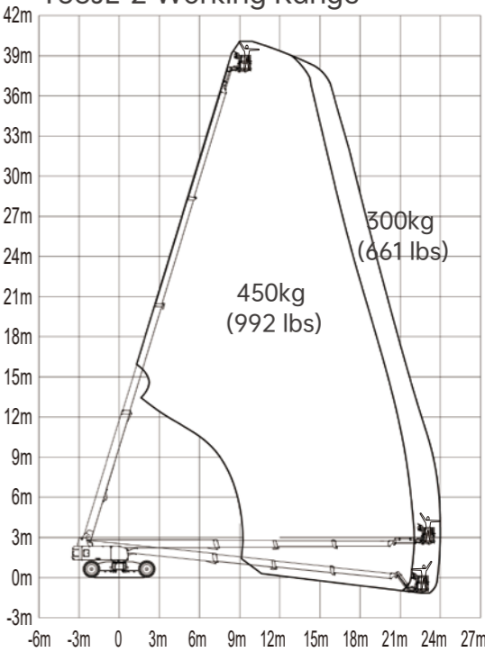
T38JE-2 Working Range
