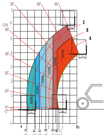
Load curve of H625 under RT condition
